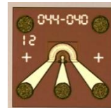
56Gbaud PIN Photodiode Chip
